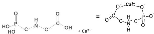
Figure 1: The distortion of the glyphosate molecule by a divalent cation like \text{Ca}^{2+}
